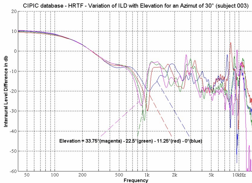
FIGURE 3 – ILD VARIATIONS FOR SUBJECT 003 (CIPIC DATABASE) [12] FOR AN AZIMUT OF 30° AND VARIOUS ELEVATION ANGLES
