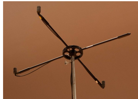
FIGURE 7 – 2 ND LAYER ARRAY (3 MICROPHONES) FIGURE OF EIGHT ELEVATION ARRAY DIRECTIVITY AXIS IS AT 90° TO BODY OF MICROPHONE
